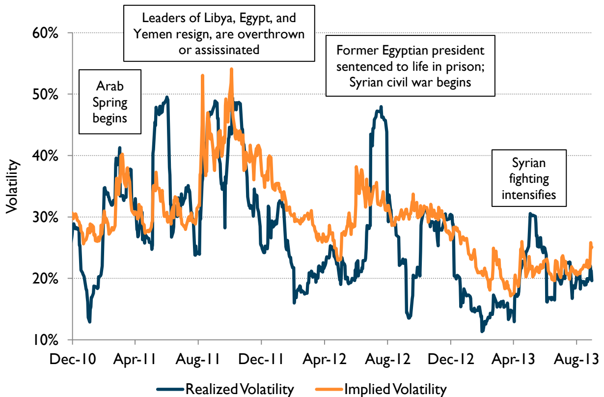
Figure 1: Realized volatility of crude oil front month futures returns using a 21-day window and 2-mo at-the-money (ATM) implied volatility of oil options.
