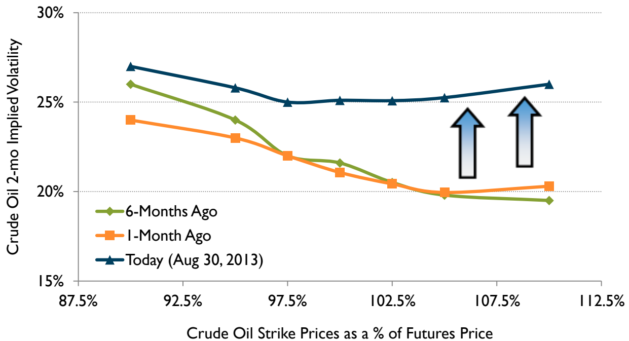
Figure 2: Crude oil option skew snapshots. We look at the implied volatility of oil options at different points in time and across different strike prices.
